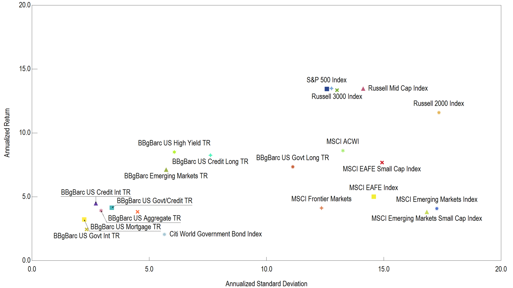
Annualized Return vs. Annualized Standard Deviation 10 Years Ending August 31, 2019
