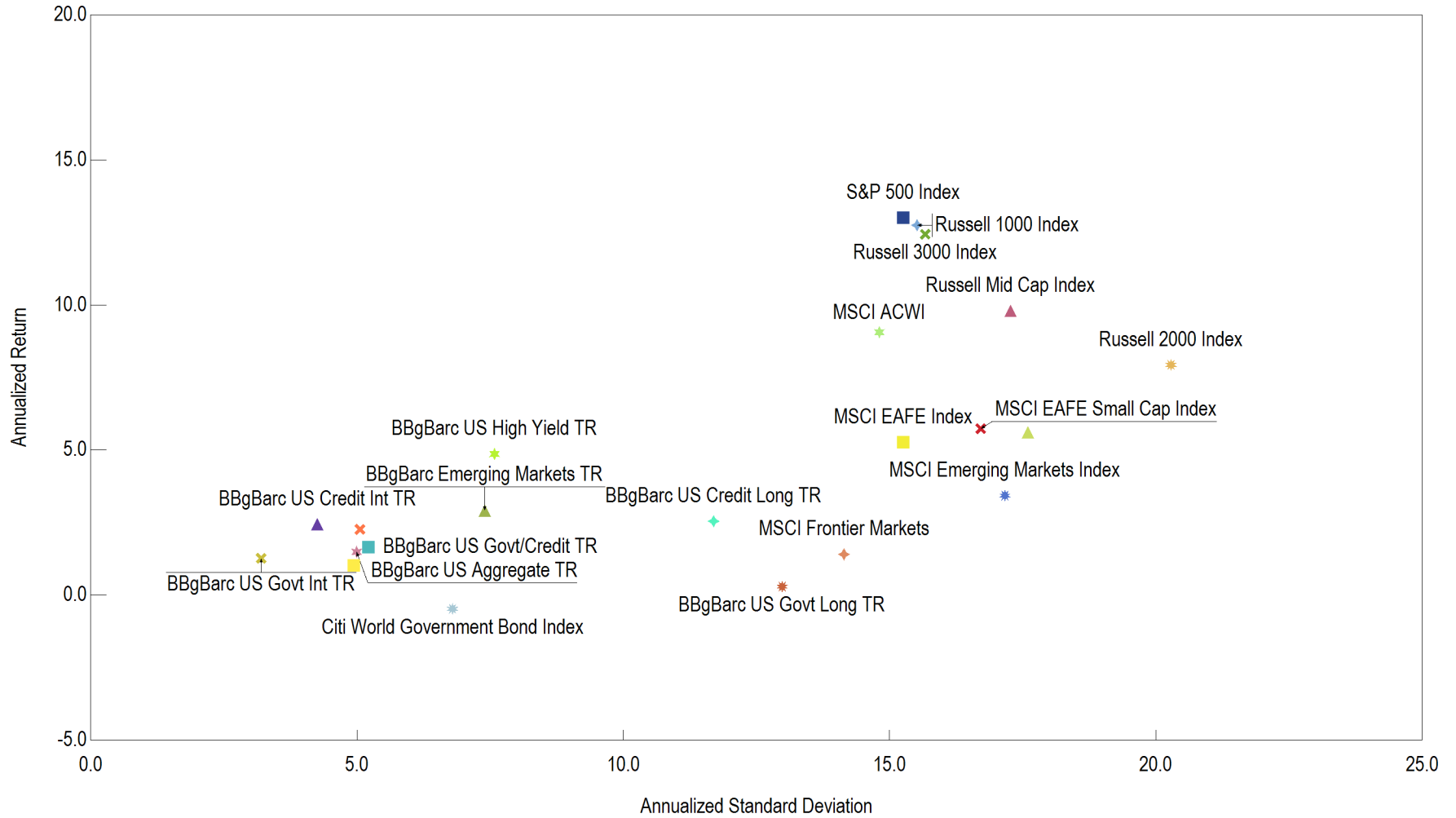
Annualized Return vs. Annualized Standard Deviation 10 Years Ending October 31, 2024
