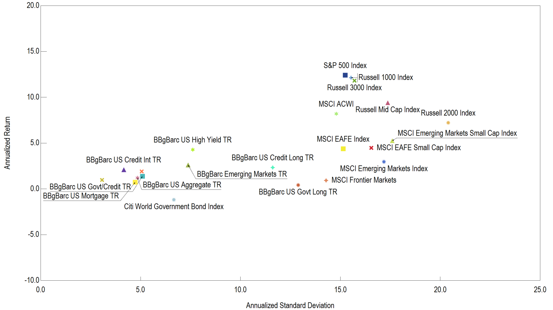
Annualized Return vs. Annualized Standard Deviation 10 Years Ending April 30, 2024
