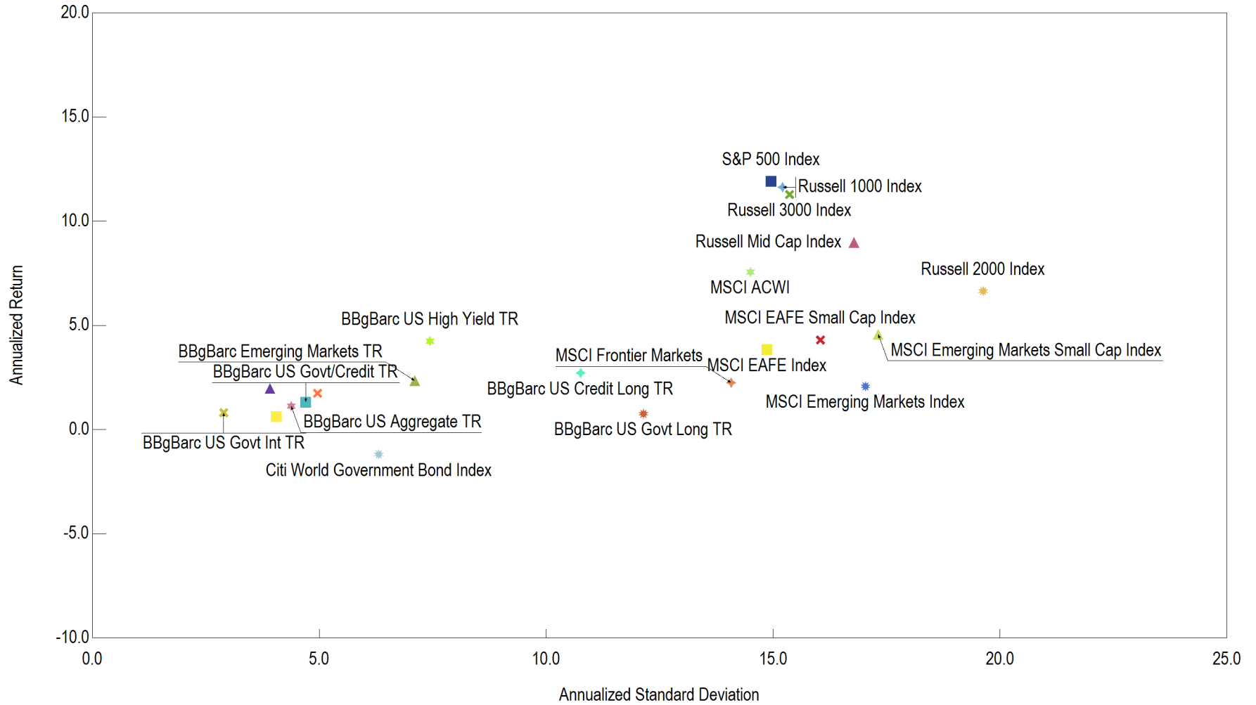
Annualized Return vs. Annualized Standard Deviation 10 Years Ending September 30, 2023
