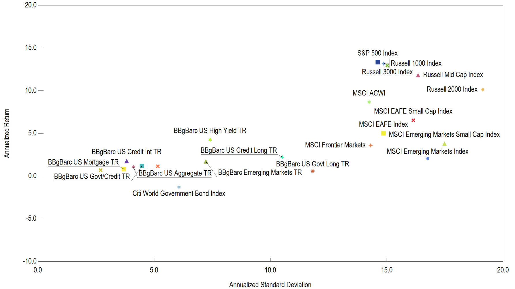
Annualized Return vs. Annualized Standard Deviation 10 Years Ending November 30, 2022
