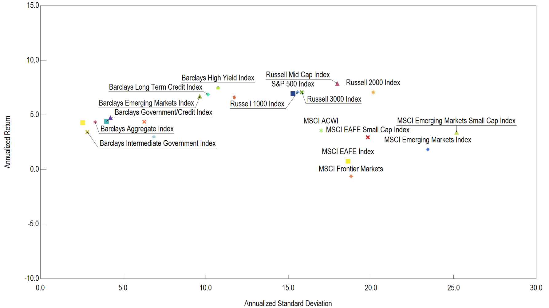
Annualized Return vs. Annualized Standard Deviation 10 Years Ending December 31, 2016
