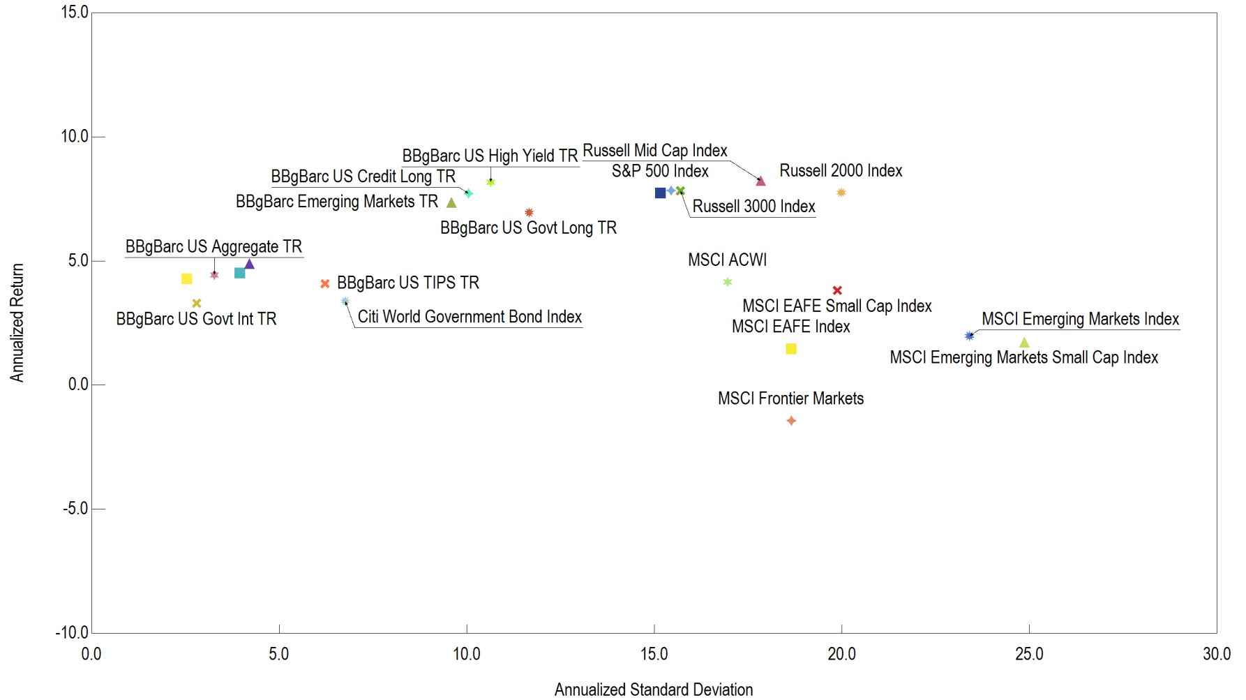
Annualized Return vs. Annualized Standard Deviation 10 Years Ending July 31, 2017
